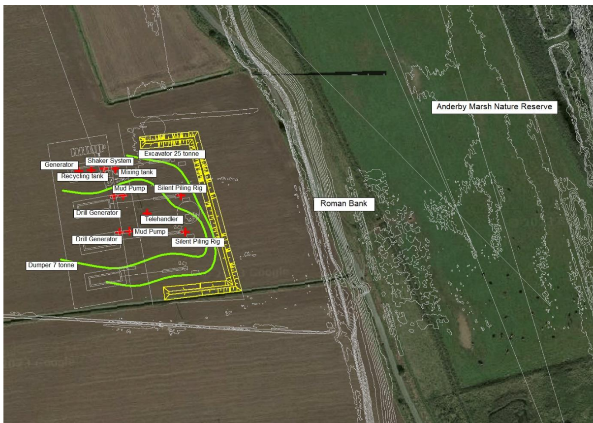
Plate 26.3: Modelled Landfall Layout
